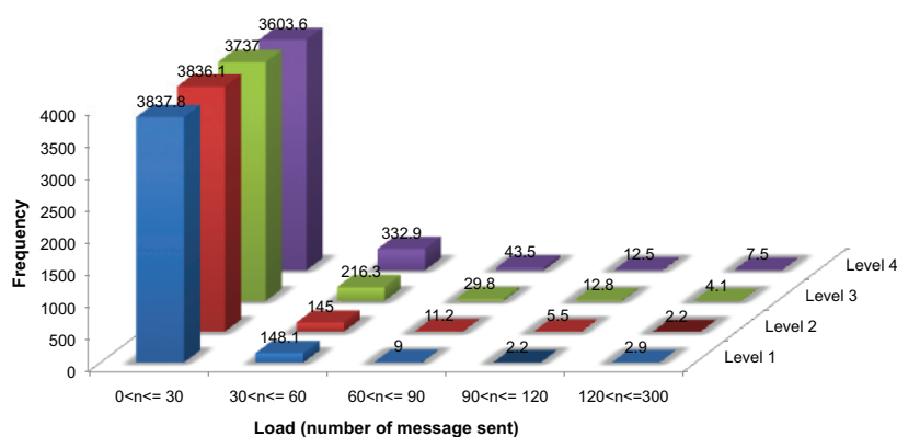
Figure 10. Load balance for communication messages (averaged over 10 networks of 4000 nodes and 10 consecutive evolution).
