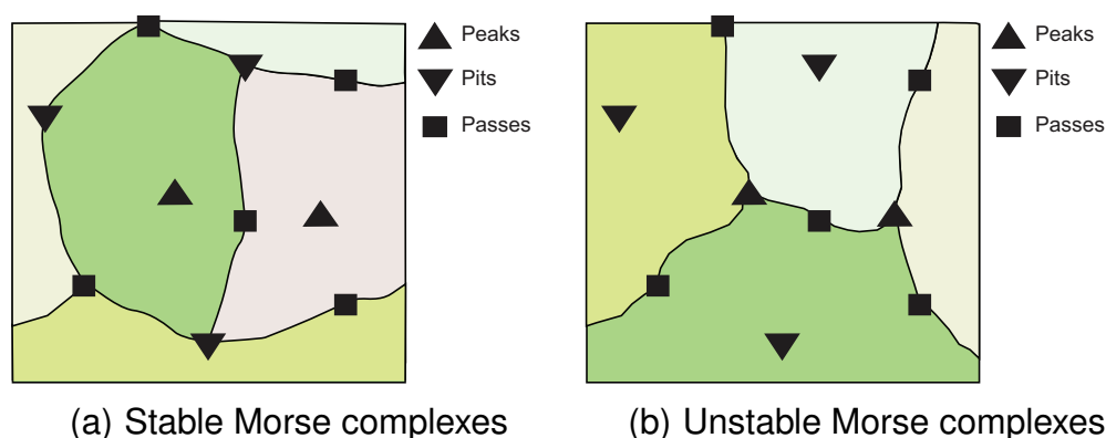
Figure 3. Stable/Unstable Morse complexes. This figure is adapted from [30].
