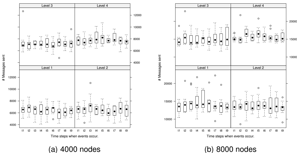
Figure 7. Number of messages generated by spatial events at each evolution step: dots are deemed to be outliers.
