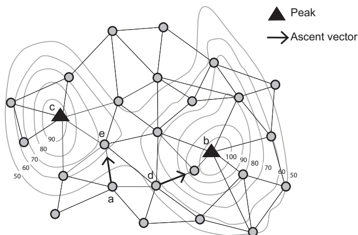
Figure 9. Example asynchronous update problem. The node a was previously a peak.
