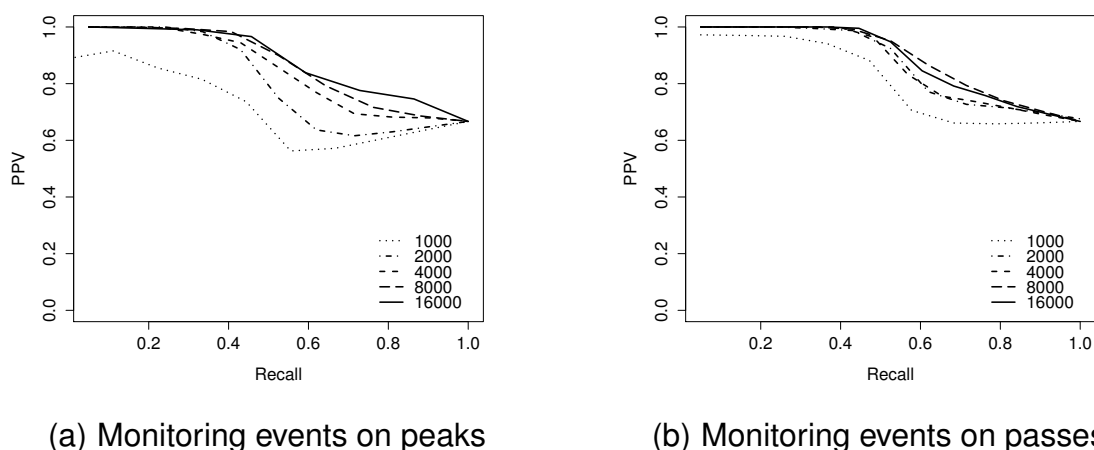
Figure 11. Positive predictive value (PPV)-recall curves for network sizes of 1000–16,000 nodes on a Level 4 surface.
