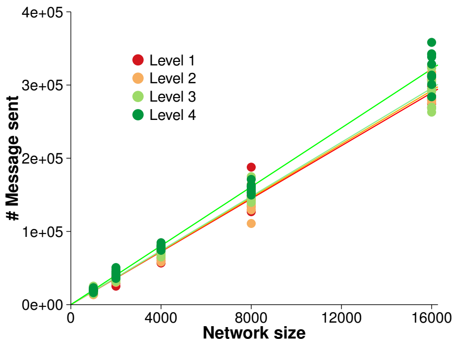
Figure 6. Overall scalability for monitoring events (averaged over 10 randomized networks and 10 consecutive time steps in each evolution).
