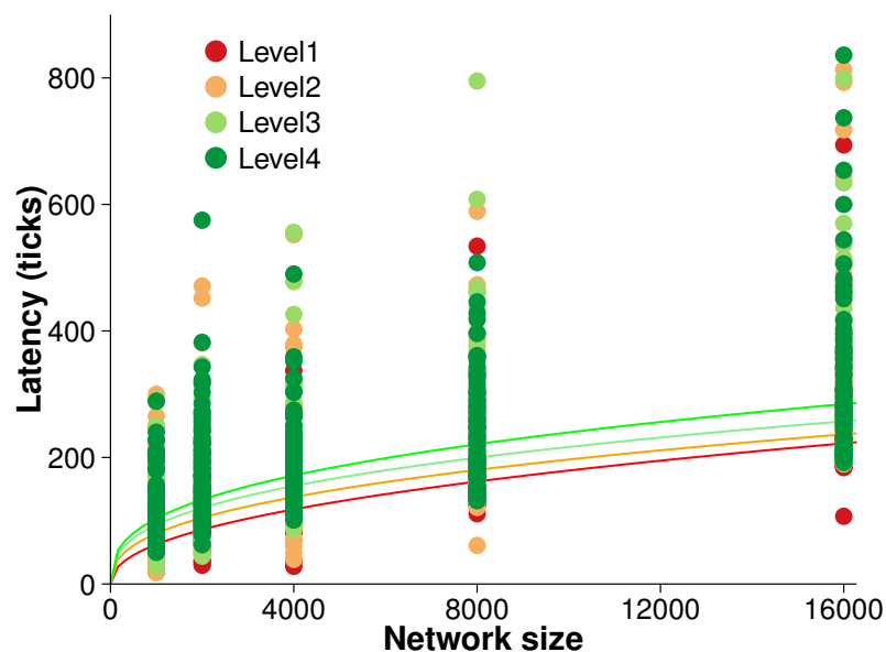
Figure 8. Latency (averaged over 10 randomized networks and 10 consecutive evolution).
