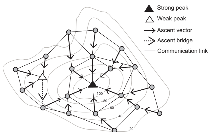
Figure 1. Identification of a strong and a weak peak, ascent vectors and an ascent bridge (Contour lines describe a scalar field showing the difference in elevation between consecutive contour lines. The sensed values can be estimated using a contour map).
