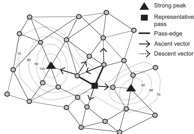
Figure 2. Representative pass (Contour lines describe a scalar field showing the difference in elevation between consecutive contour lines. The sensed values can be estimated using a contour map.)
